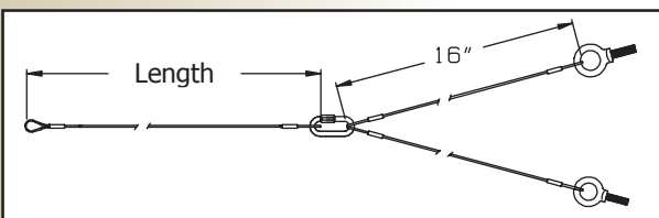
D = One with loop on both ends = Two 16" cables with eyebolt on one end and loop on the other end
