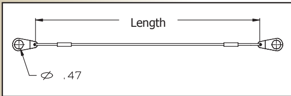
A = Retaining washers on both ends
